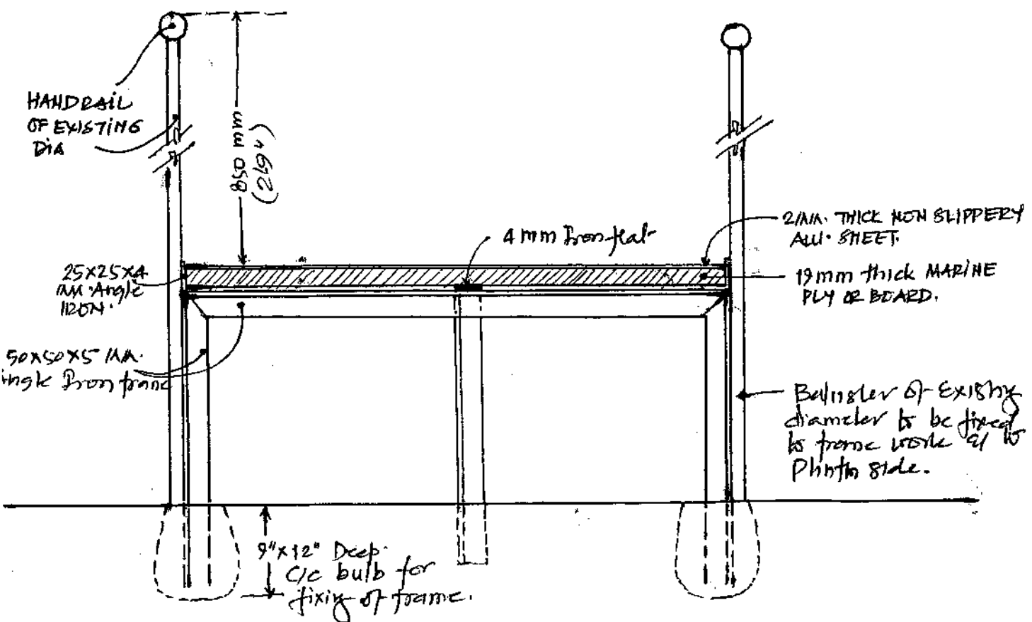
DETAIL OF FIXING OF ANGLE IRON FRAME FOR RAMP
